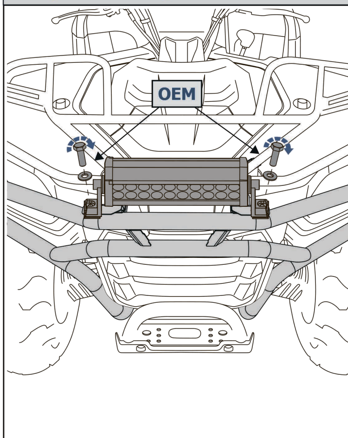
Optional LED light bar installation
